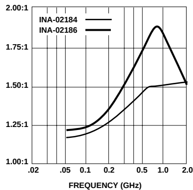
Figure 7. Input VSWR vs. Frequency, I_d = 35\text{ mA} .
