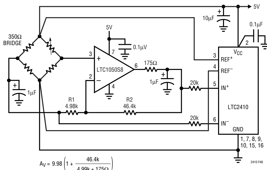
Figure 48. Bridge Amplification Using a Single Amplifier
