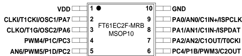
Figure 1-5 MSOP10
