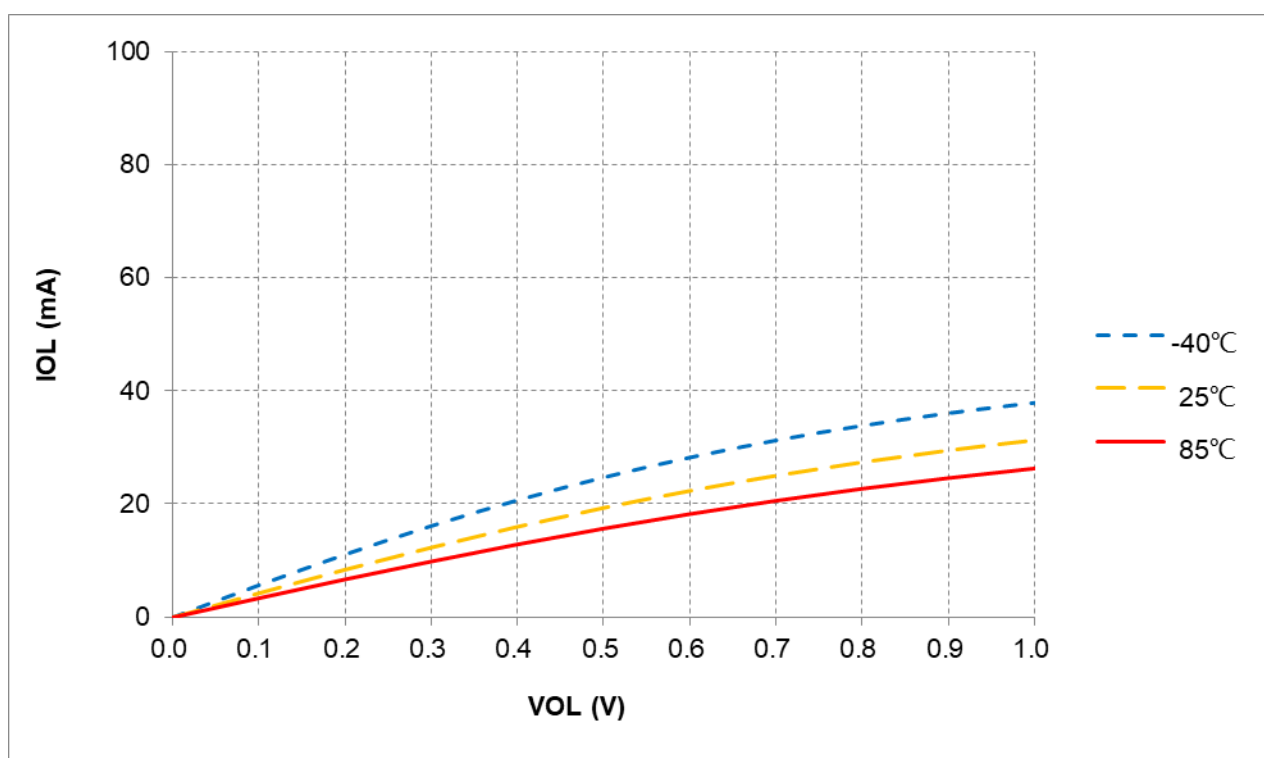
Figure 19-6 I_{OL} vs. V_{DD} , V_{OL} @ L = 19\text{mA}
