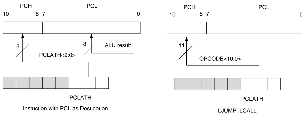
Figure 17-3 Loading of PC in different situations
