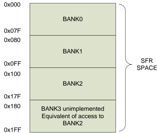
Figure 17-2 Indirect addressing
