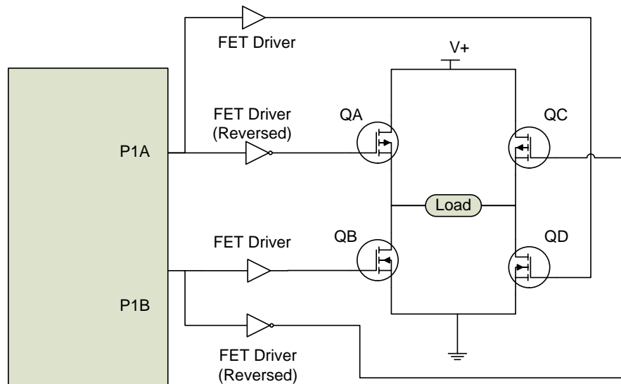
Figure 10-8 Half-Bridge Output Driving a Full-Bridge Circuit (2PMOS+2NMOS, P1A~P1B active high)
