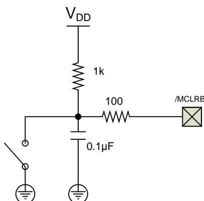
Figure 4-3 /MCLRB reset circuit
