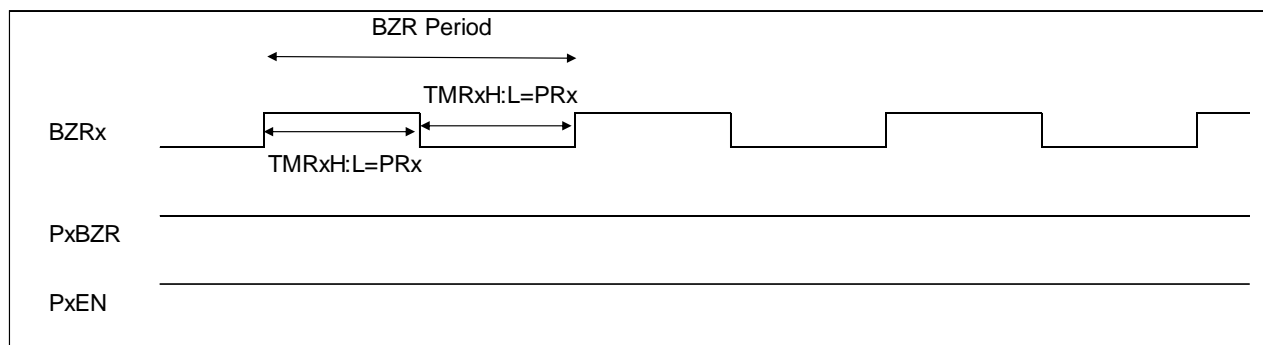
Figure 7-4 50% duty cycle of the BUZZER square wave
