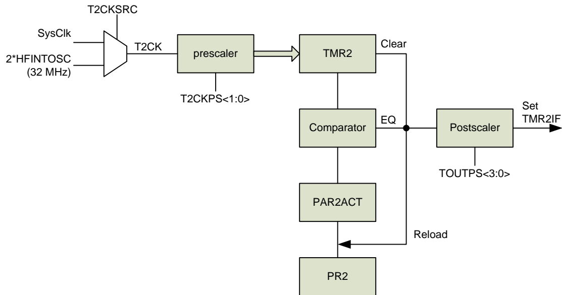
Figure 7-3 Timer2 block diagram
