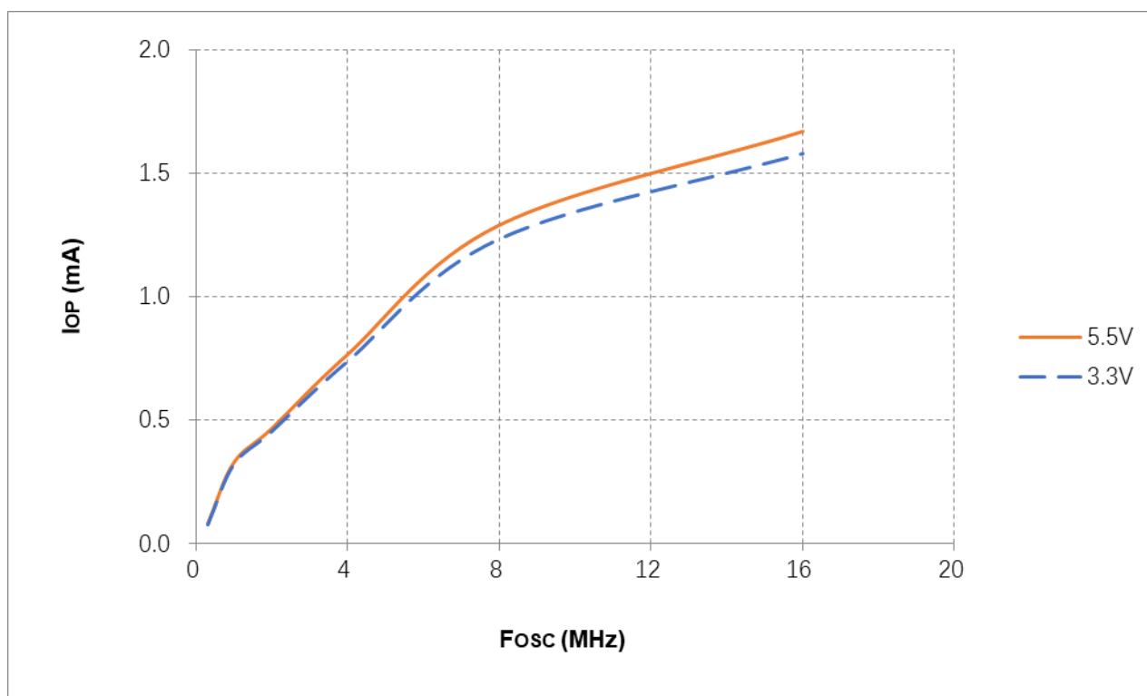
Figure 19-3 I_{DD} vs. Frequency (2T, T_A = 25^\circ\text{C} )
