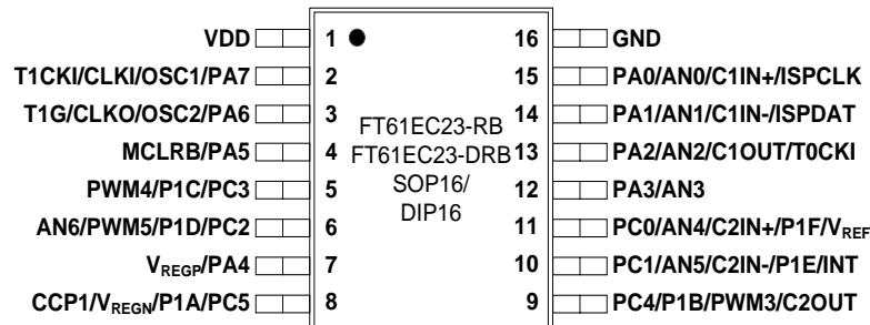
Figure 1-7 SOP16 / DIP16
