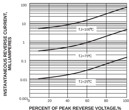
FIG. 4-TYPICAL REVERSE CHARACTERISTICS
