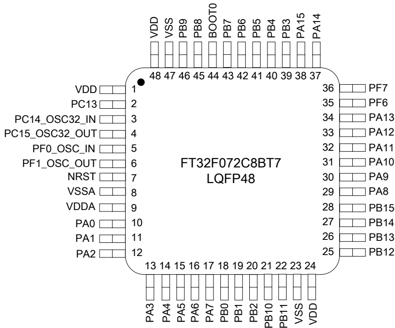
Figure 4.4 LQFP48(B) package pinout
