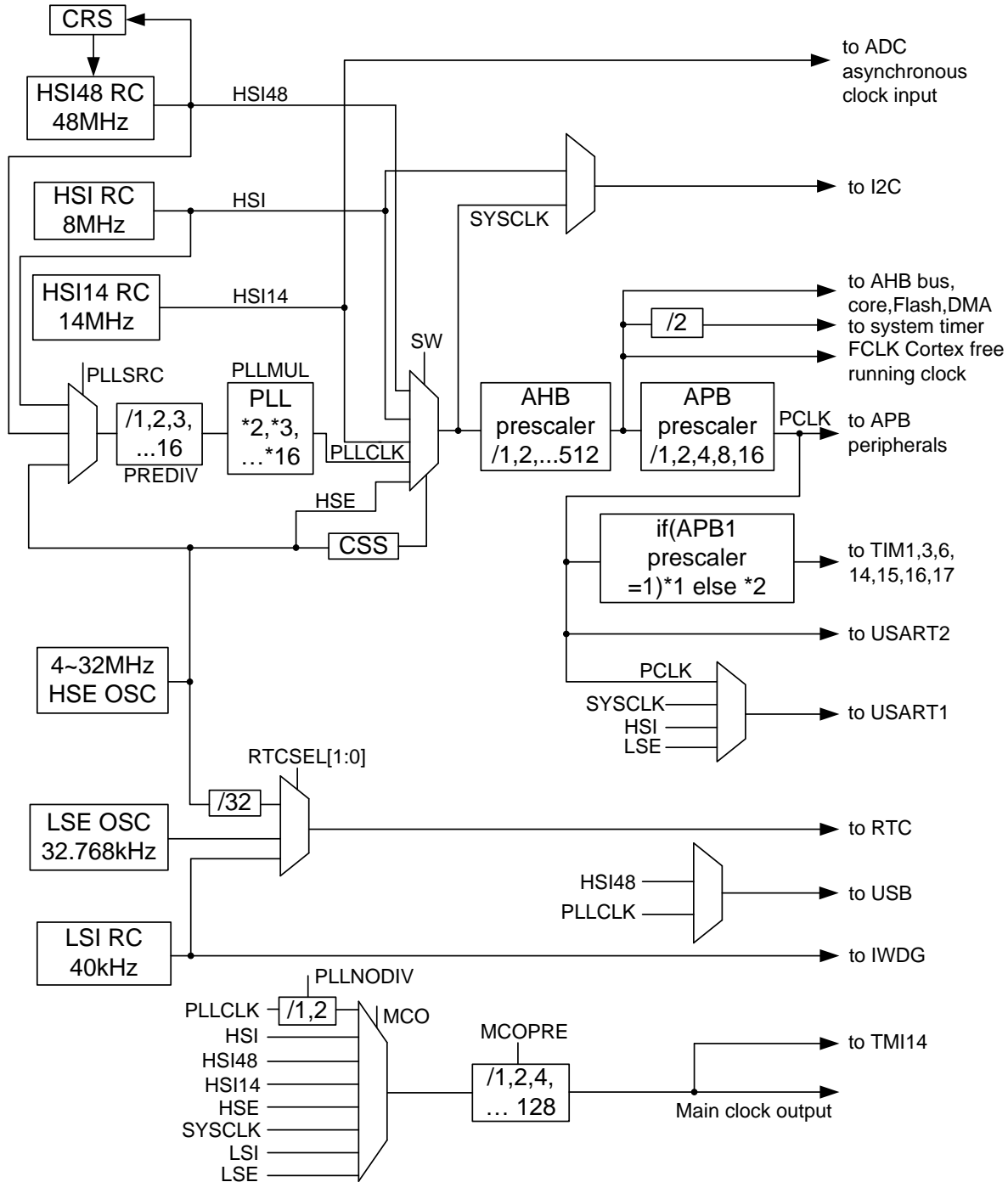
Figure 3.1 Clock tree
