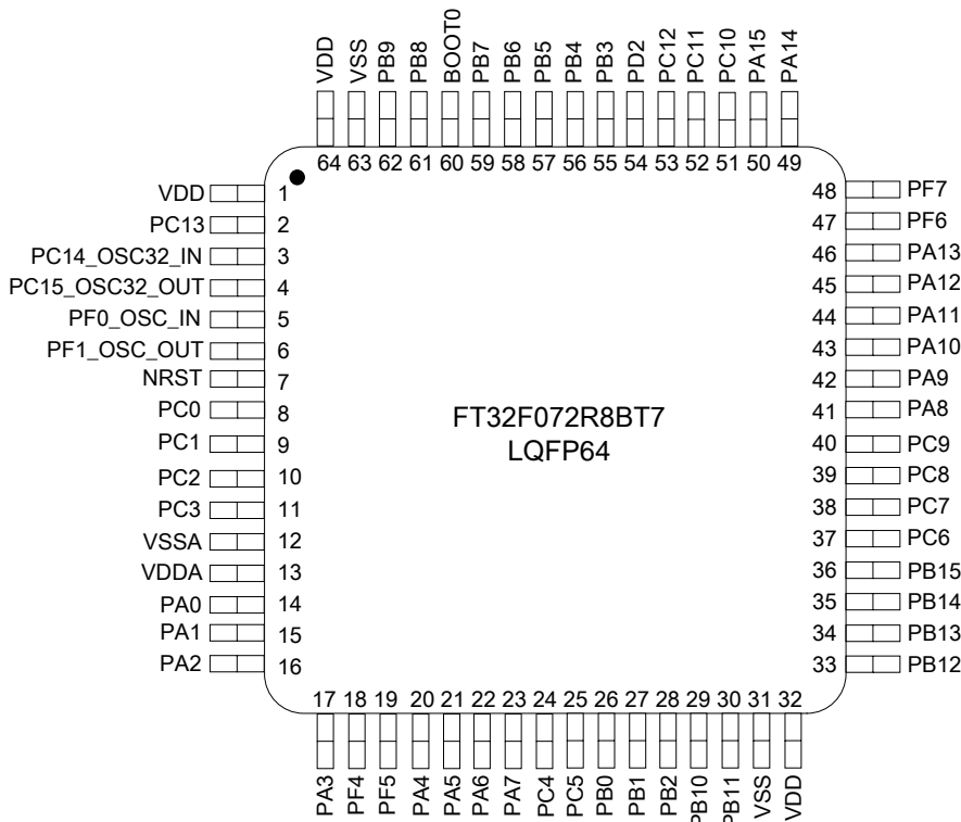
Figure 4.2 LQFP64(B) package pinout
