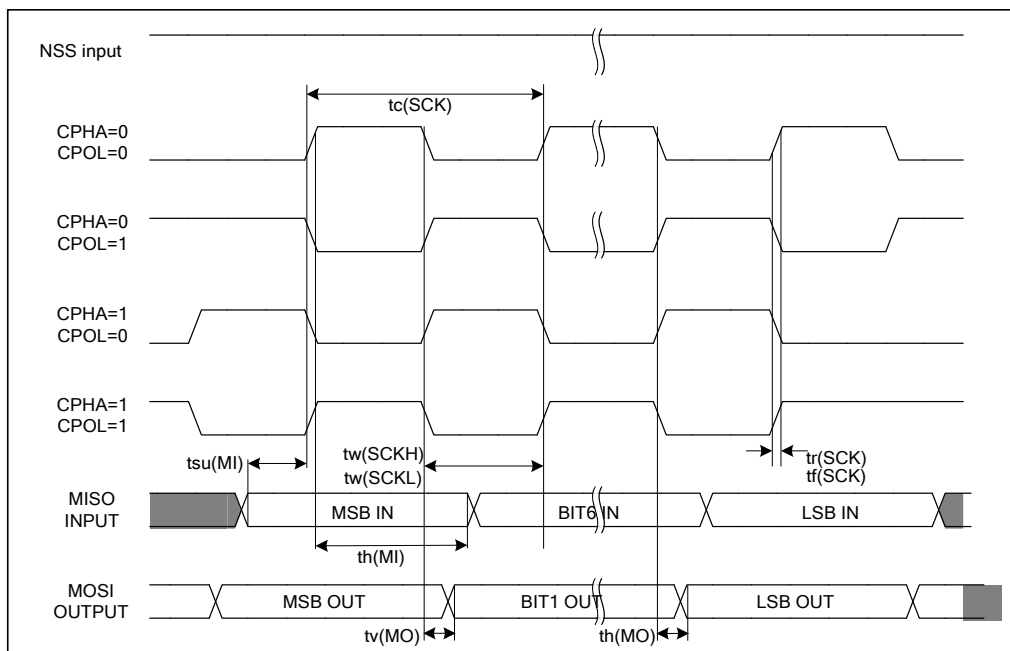
Figure 6.15 SPI timing diagram – master mode
