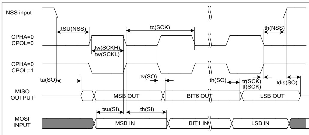
Figure 6.14 SPI timing diagram – slave mode and CPHA=1
