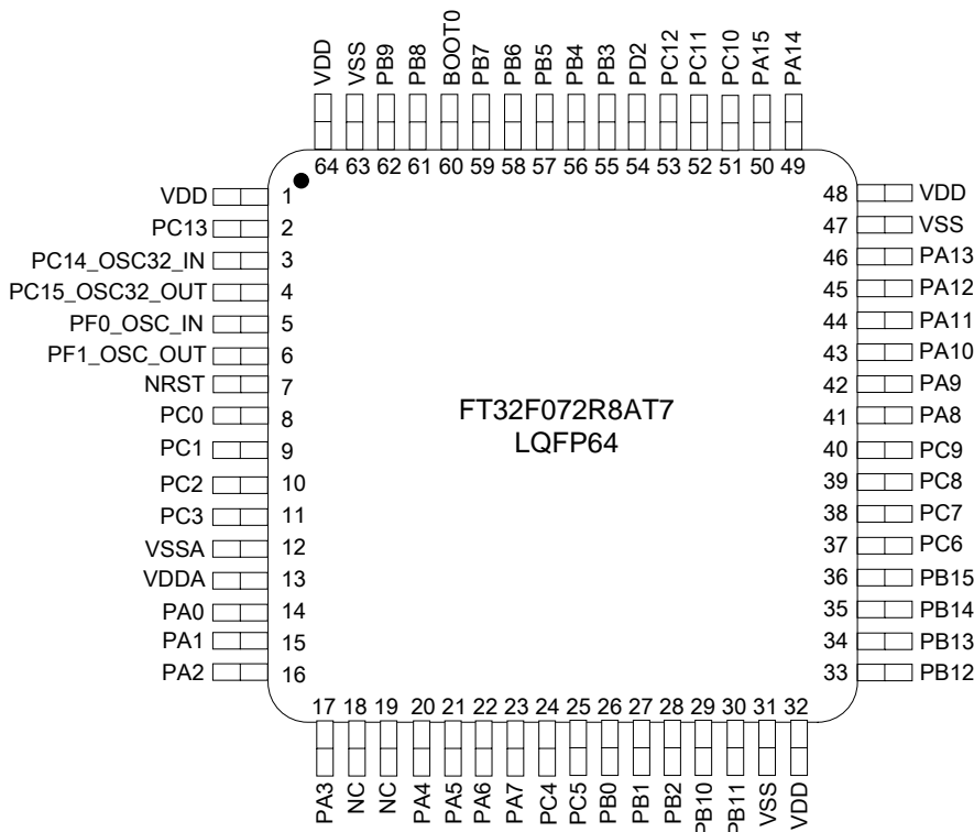
Figure 4.1 LQFP64(A) package pinout
