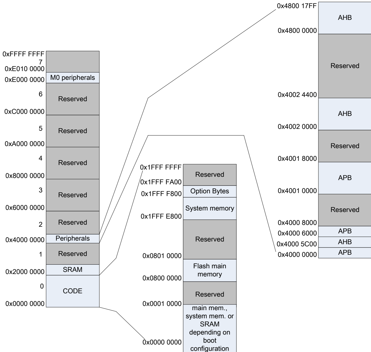
Figure 5.1 Memory map
