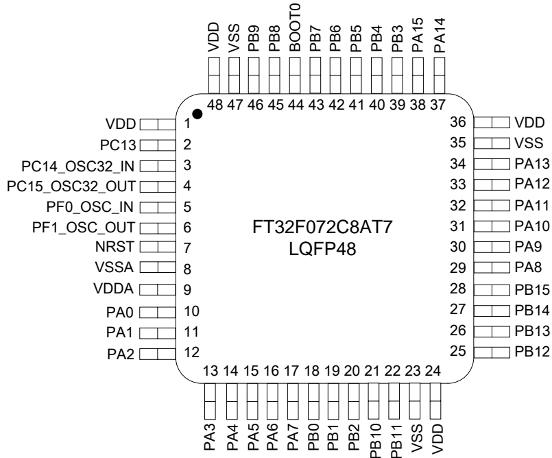
Figure 4.3 LQF48(A) package pinout
