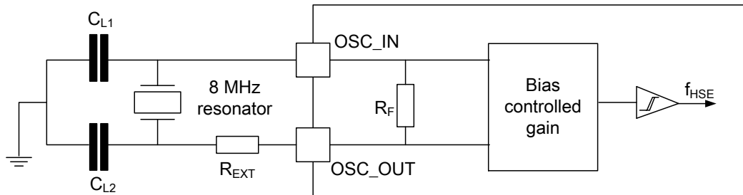
R_{EXT} value depends on the crystal characteristics
