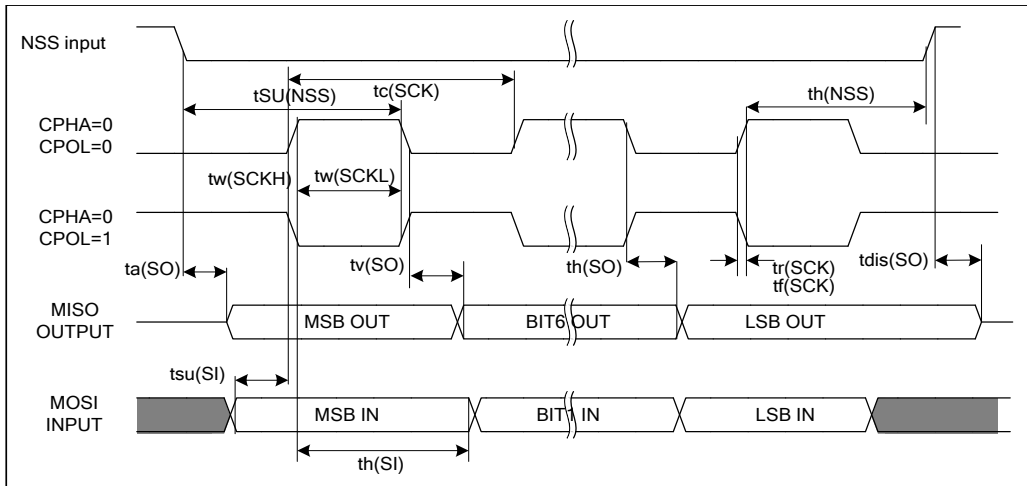
Figure 6.13 SPI timing diagram – slave mode and CPHA=0
