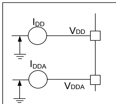
Figure 6.4 Current consumption measurement scheme
