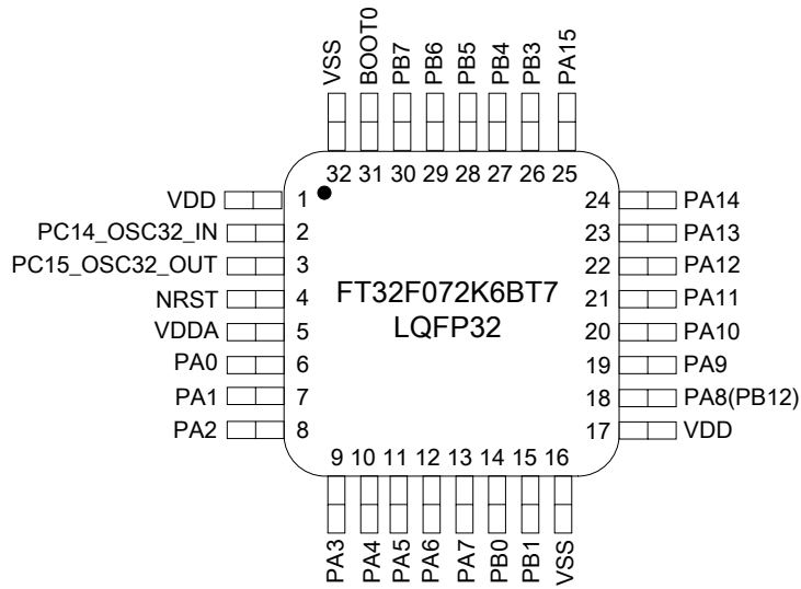
Figure 4.5 LQFP32(B) package pinout 1
