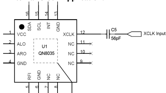
Figure 9 External Clock Input Circuit
