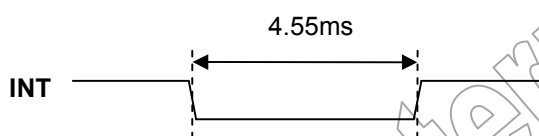
Figure 12 Interrupt Output
