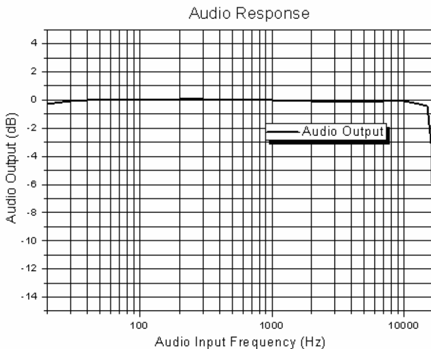
Figure 6 Audio Response
