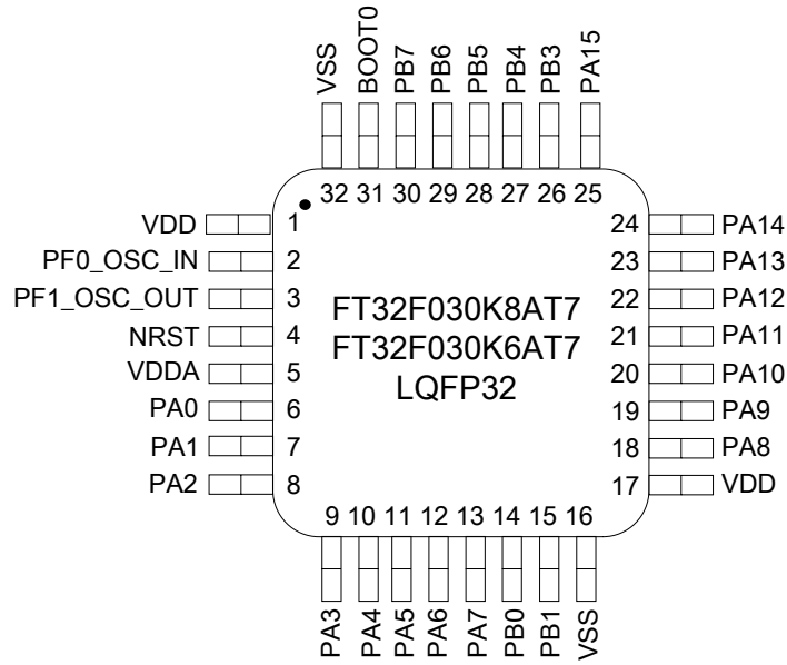
Figure 4.3 LQFP32(A) package pinout
