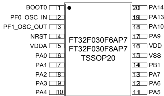
Figure 4.7 TSSOP20(A) package pinout
