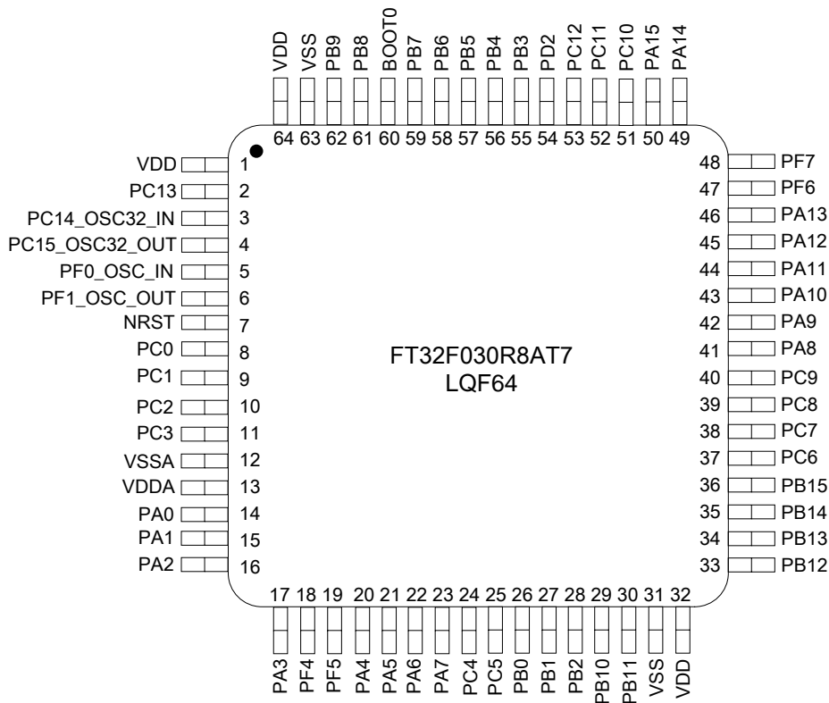
Figure 4.1 LQF64(A) package pinout
