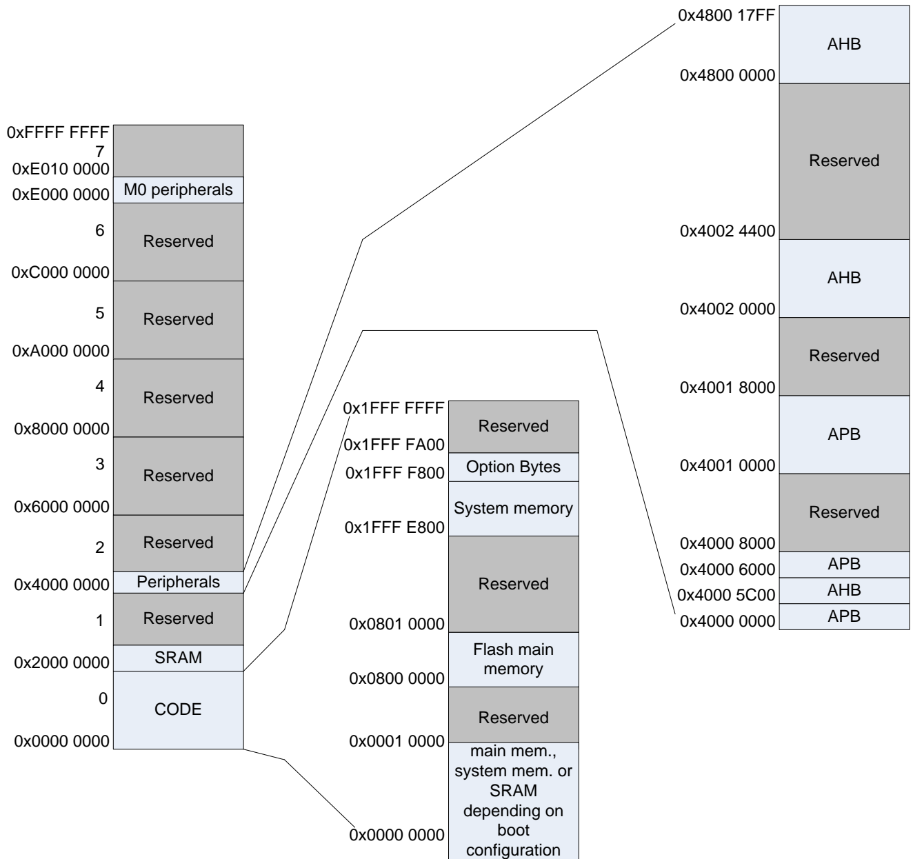
Figure 5.1 Memory map
