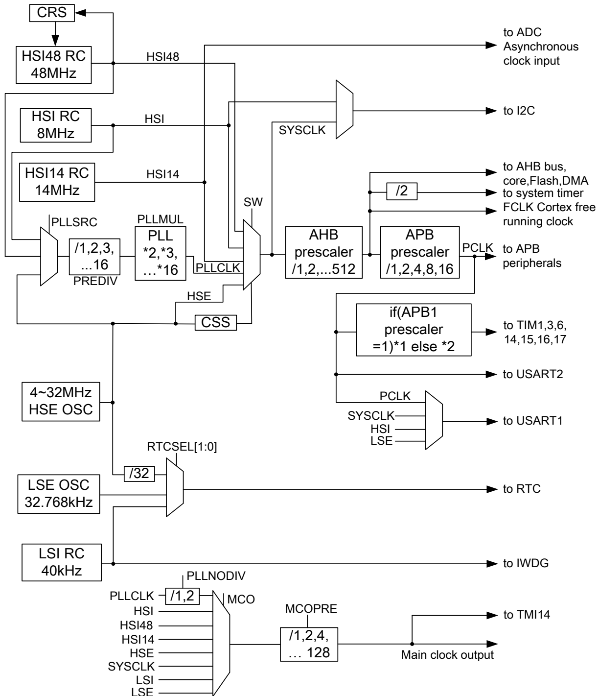
Figure 3.1 Clock tree
