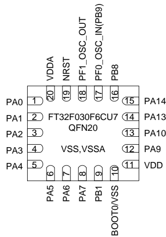
Figure 4.11 QFN20(C) package pinout 3
