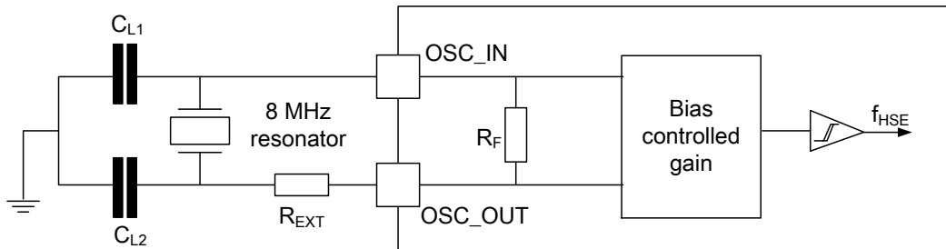
Figure 6.7 Typical application with an 8 MHz crystal
