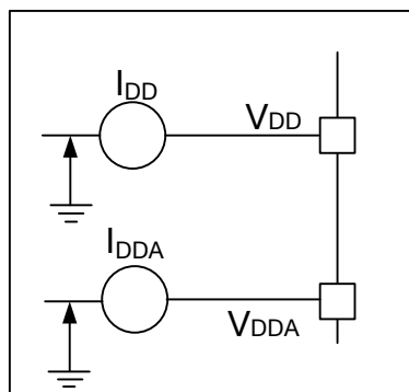
Figure 6.4 Current consumption measurement scheme
