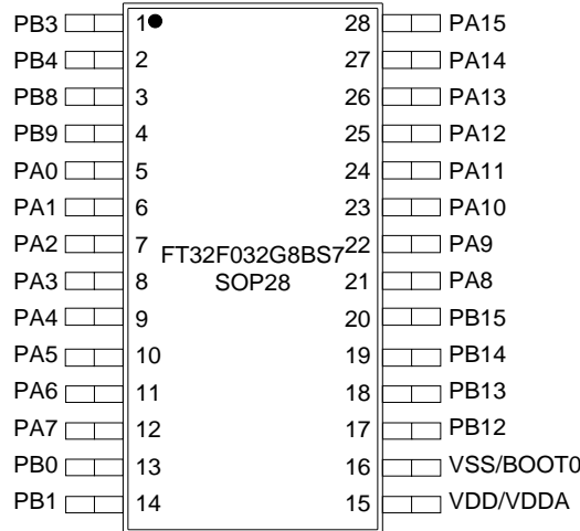
Figure 4.5 SOP28(B) package pinout
