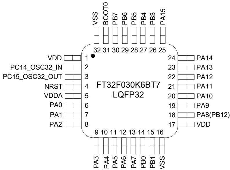
Figure 4.4 LQFP32 (B) package pinout 1
