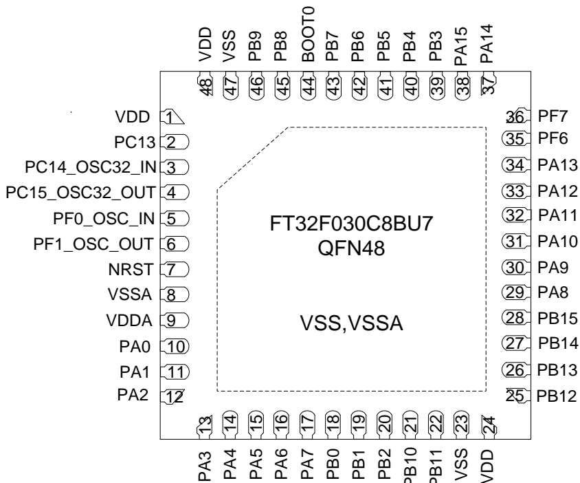
Figure 4.8 QFN48(B) package pinout
