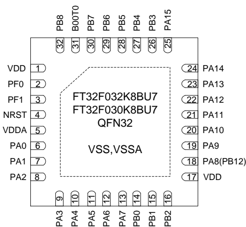
Figure 4.9 QFN32(B) package pinout 2
