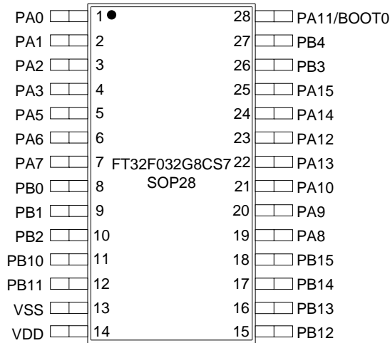
Figure 4.6 SOP28(C) package pinout
