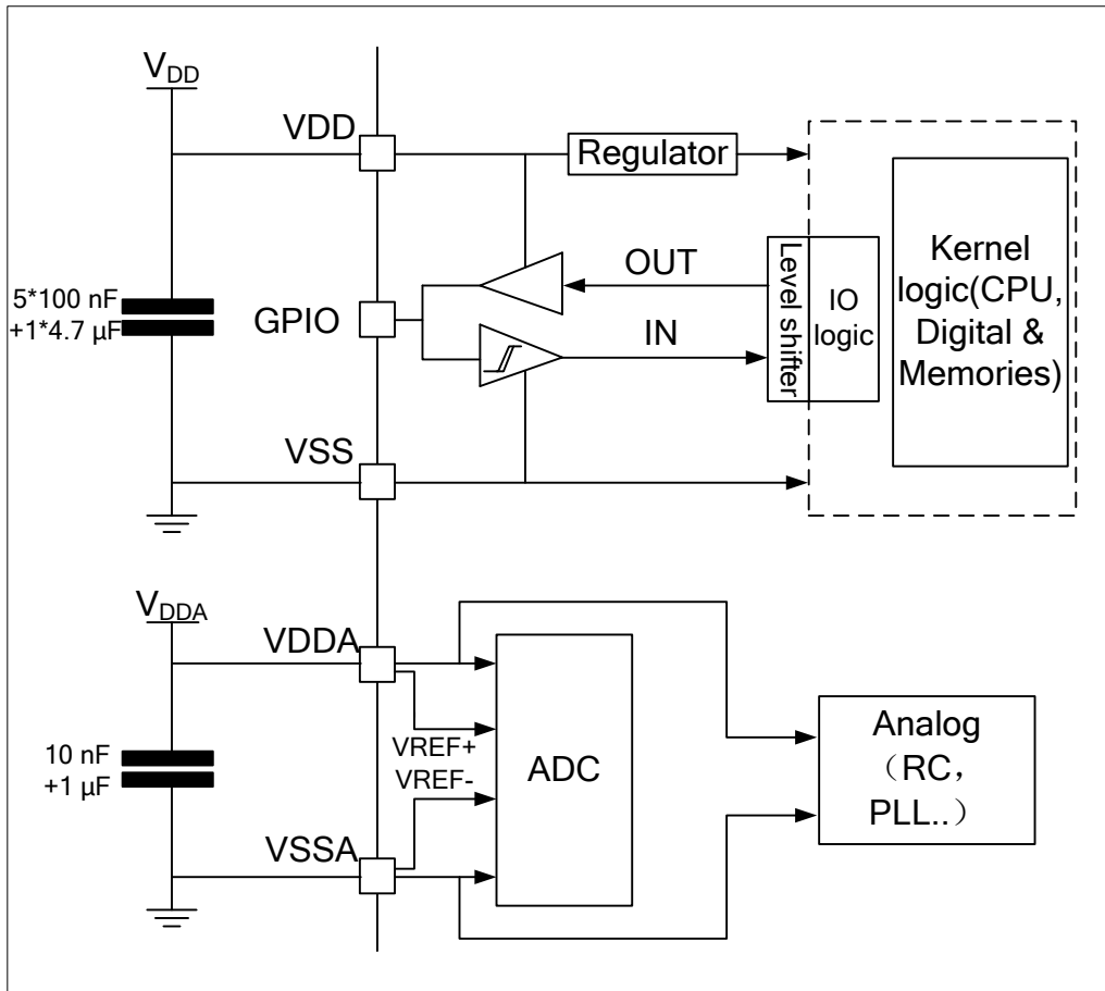
Figure 6.3 Power supply scheme
