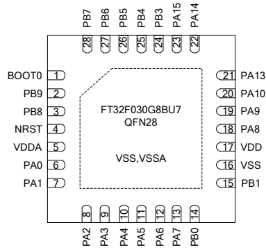
Figure 4.10 QFN28(B) package pinout
