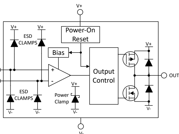
Figure 7-2. TLV181x-Q1 Push-Pull Block Diagram
