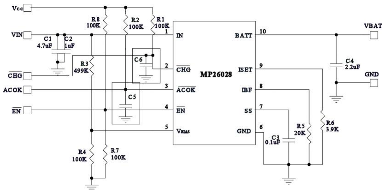
Figure 5—Filtered Charge Status & Input Power Good Interface
