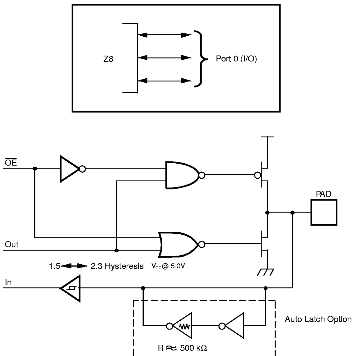
Figure 7. Port 0 Configuration
