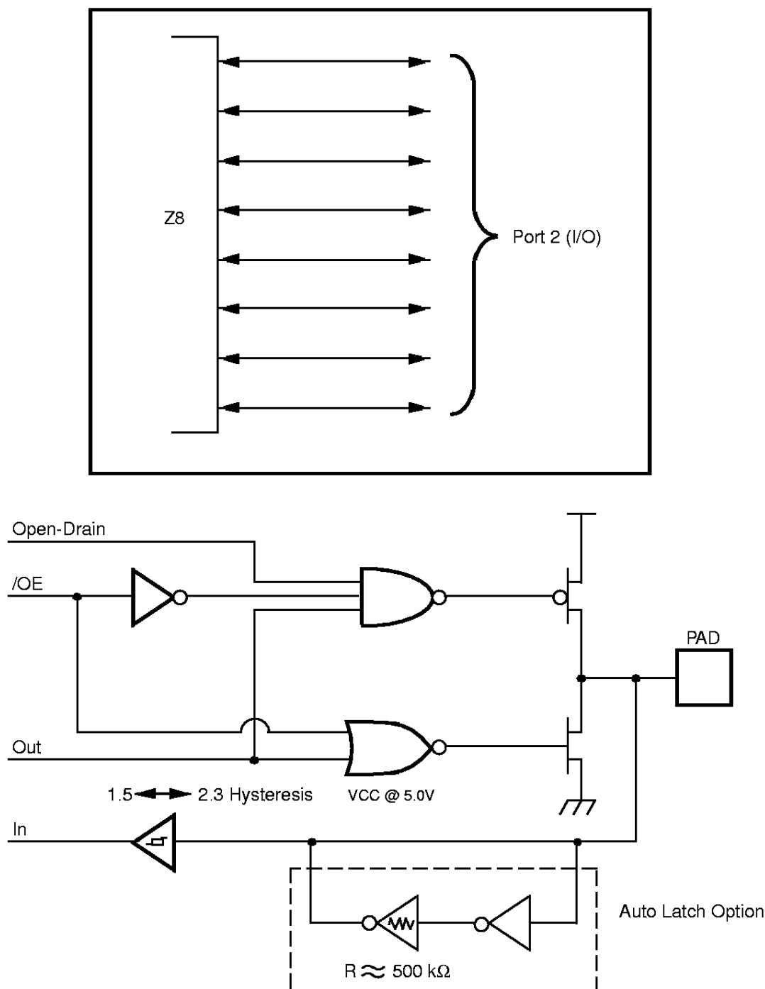
Figure 8. Port 2 Configuration
