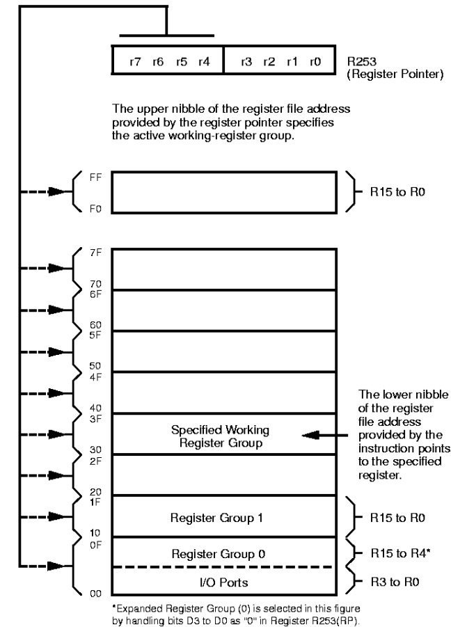
Figure 13. Register Pointer
