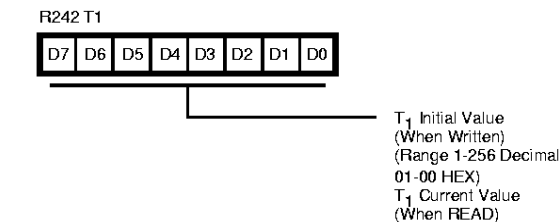
Figure 25. Counter Timer 1 Register (F2 H : Read/Write)
