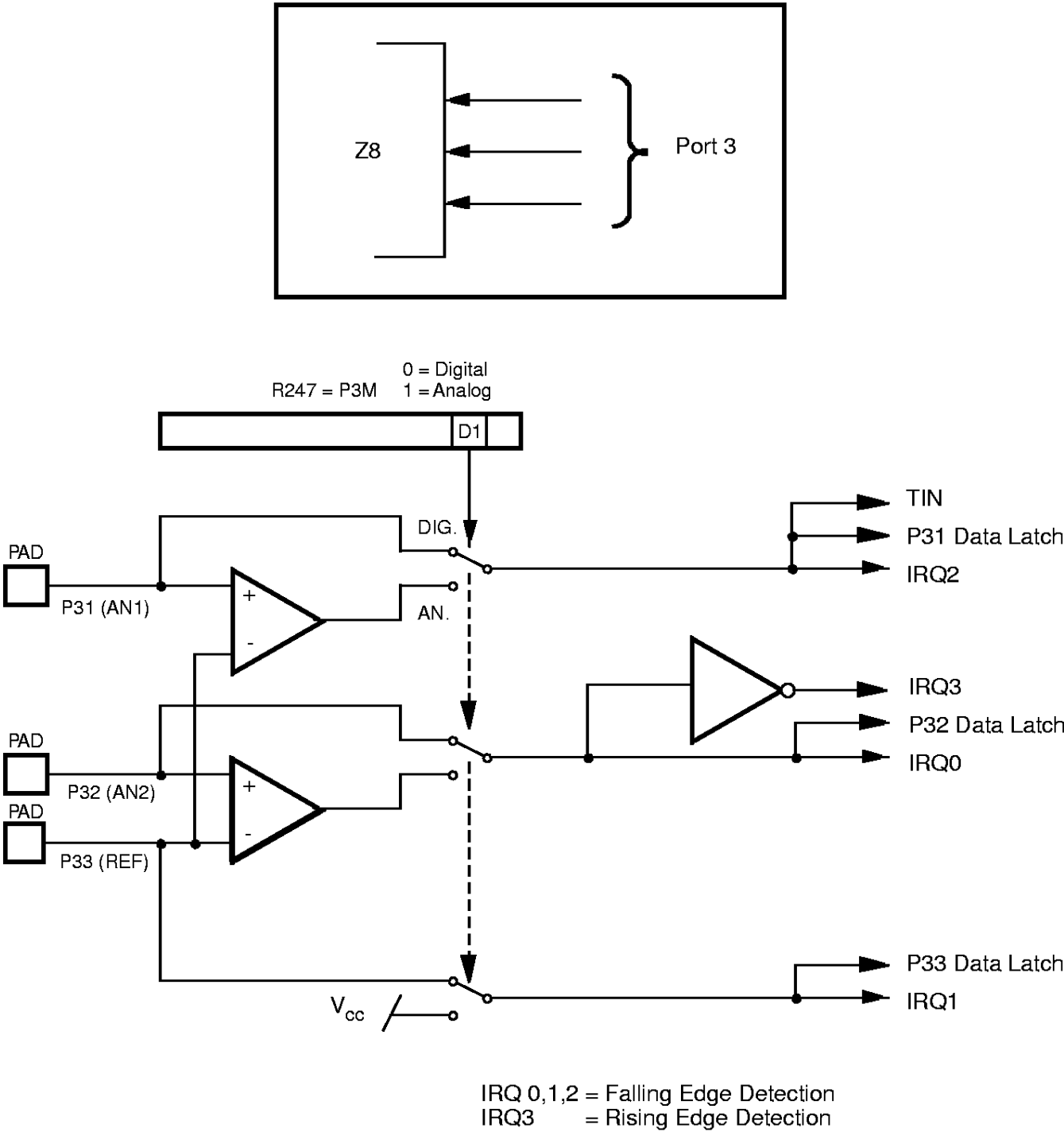
Figure 9. Port 3 Configuration
