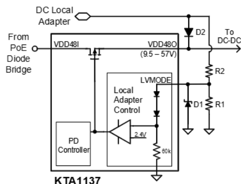
Figure 19. LVMODE Implementation
