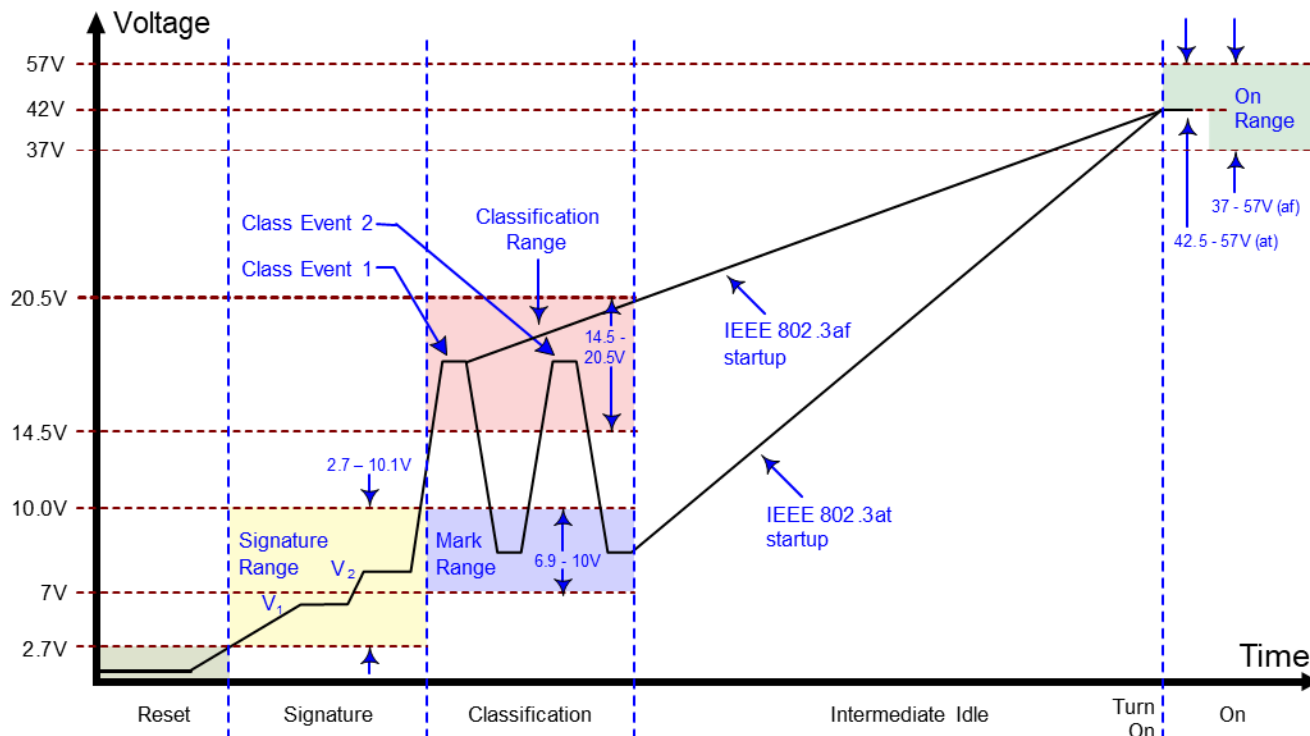
Figure 21. 802.3at Typical Power-On Waveform
