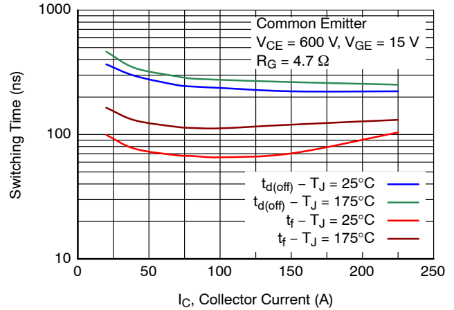
Figure 14. Turn-Off Switching Time vs. Collector Current
