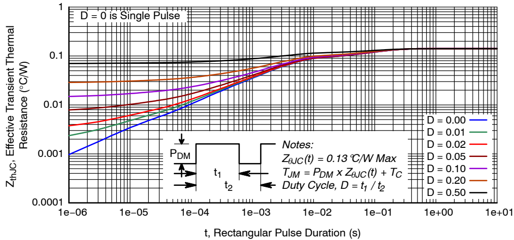
Figure 20. Transient Thermal Impedance of IGBT
