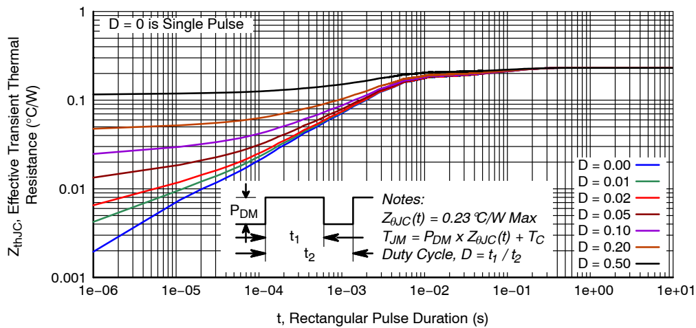
Figure 21. Transient Thermal Impedance of Diode
