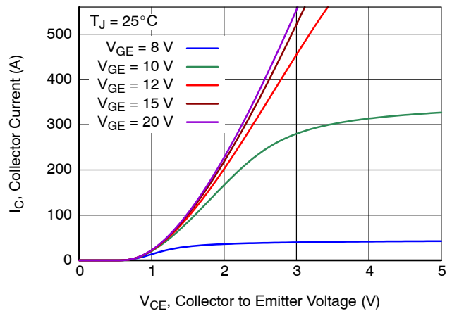
Figure 2. Output Characteristics
