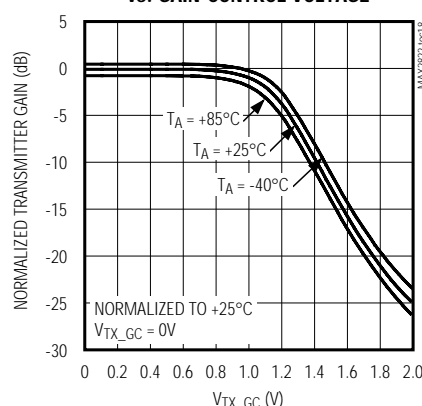
TRANSMITTER GAIN vs. GAIN-CONTROL VOLTAGE
