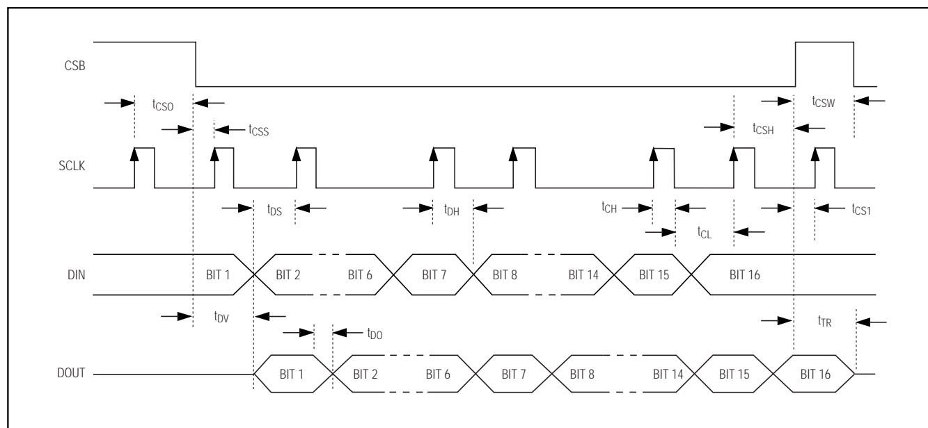
Figure 1. MAX2822 Serial Interface Timing Diagram
